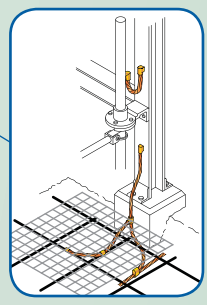
ERITECH ® Prefabricated Mesh for Switch Shaft and Operating Handle Grounding
